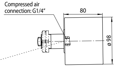
Thruster 065
