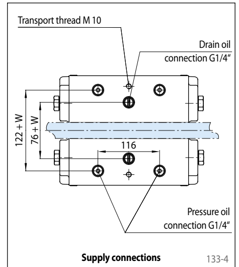
Dimensions of customer connecting part 133-3
