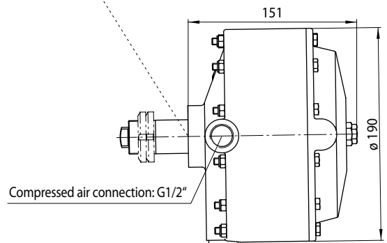
Thruster 105
