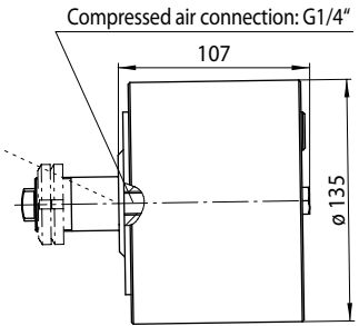
Thruster 085 and 095
